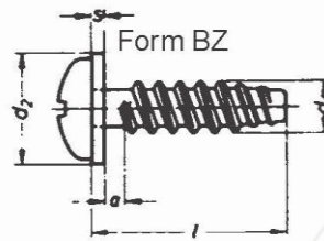
Type BZ with flat end
