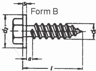
Type B with cone end
